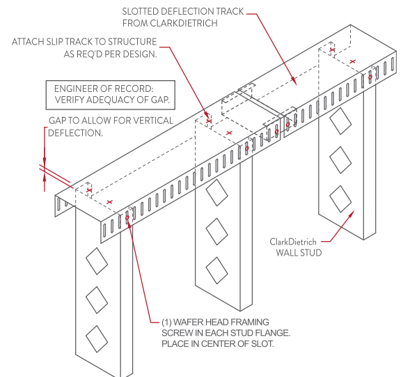
2 SLOTTED DEFLECTION TRACK DETAIL WITH TRACK SPLICE
