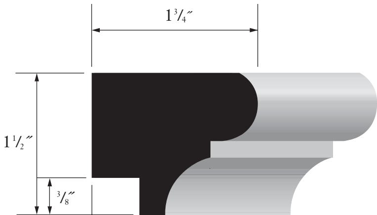
\frac{1}{2} " BBC POPLAR WAINSCOT CAP
